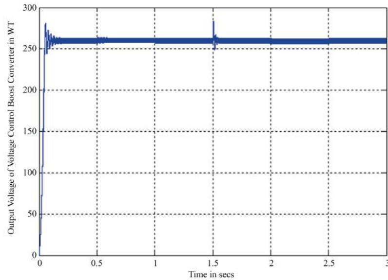
Figure 13. Output voltage of voltage control boost converter of WT.
