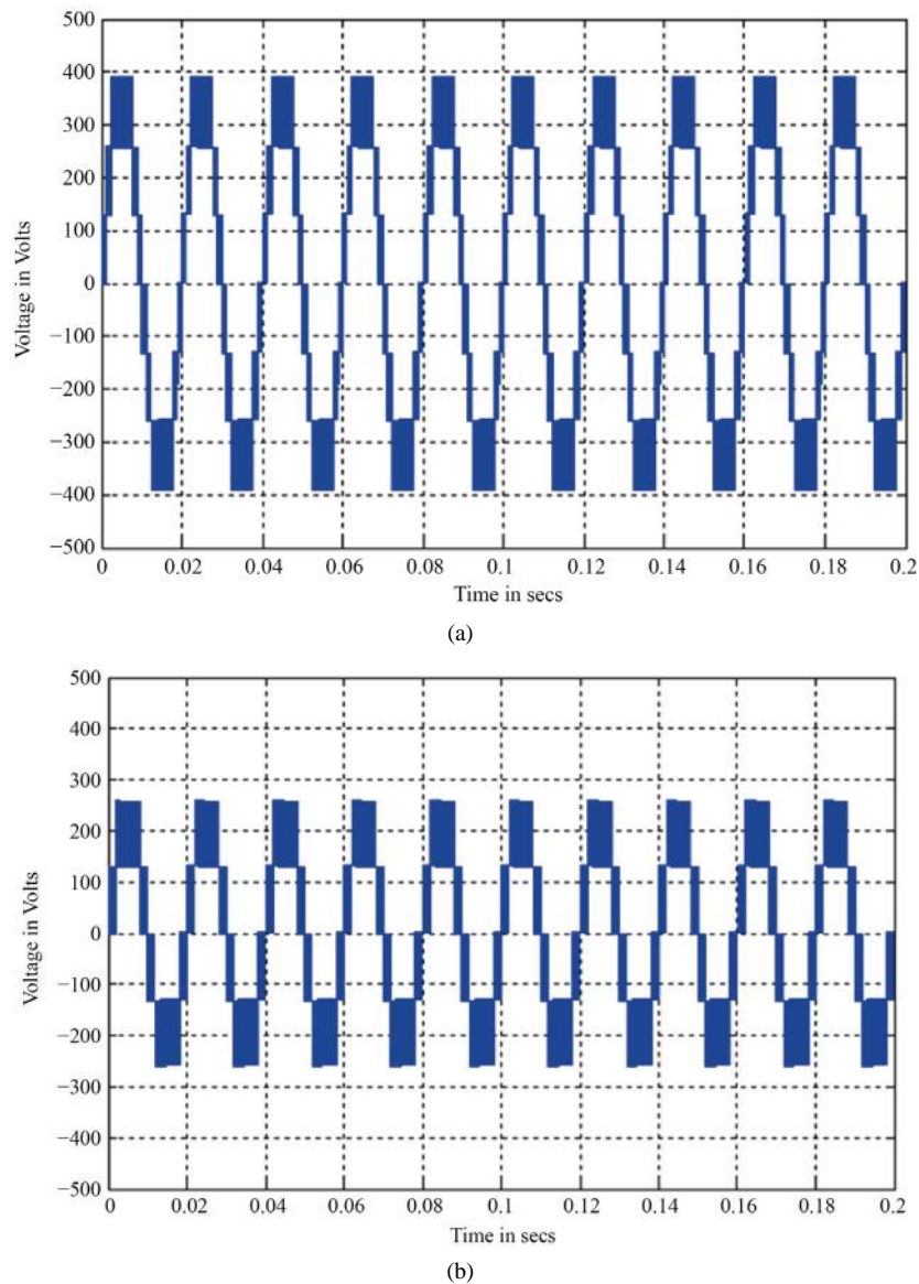
Figure 15. (a) Output voltage of proposed inverter when the modulation index is 0.95 (seven levels); (b) Output voltage of proposed inverter when the modulation index is 0.6 (five levels).
