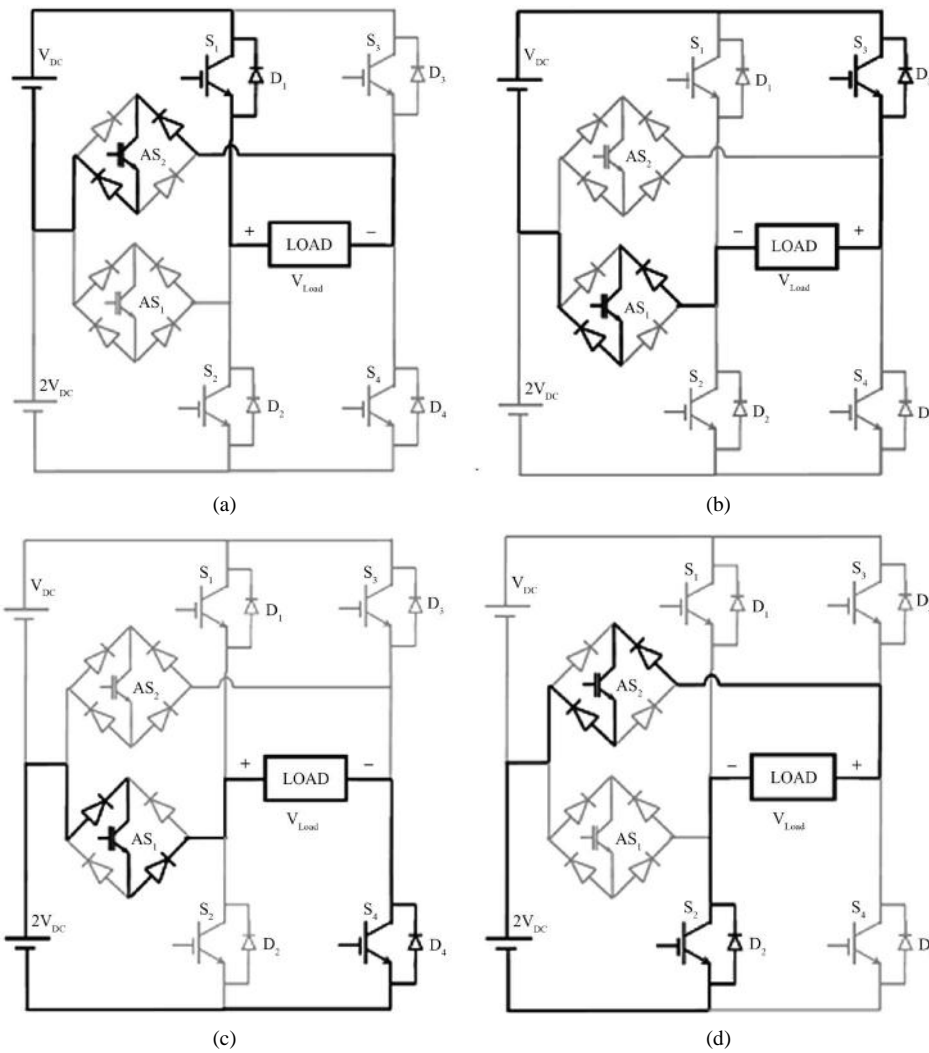
Figure 1. Proposed asymmetrical MLI topology.
