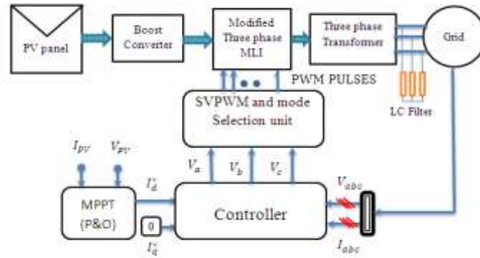
Figure 1. Block diagram of Modified three phase MLI
