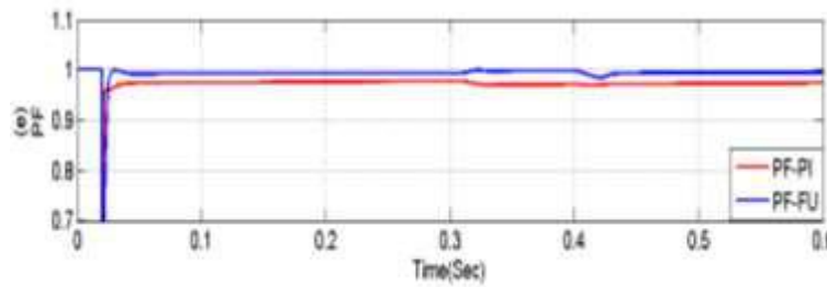
Figure 13. Power factor
