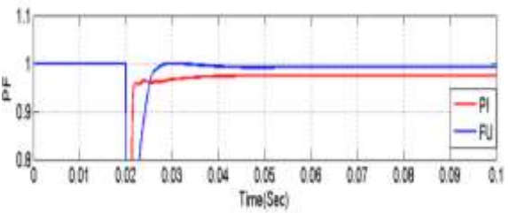
Figure 9. Power factor
